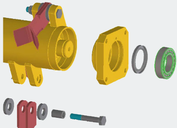
2300 RPM high speed rotor with fully enclosed bearings
