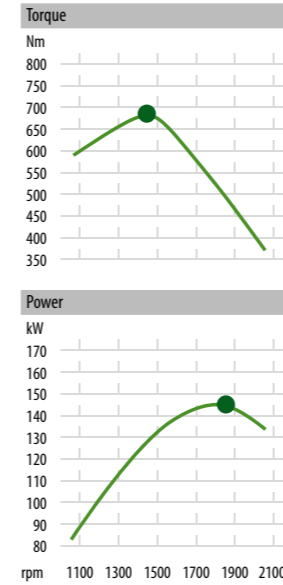
Engine characteristics – Fendt 516 Vario 687 Nm torque, 165 hp maximum output at 1,900 rpm.
